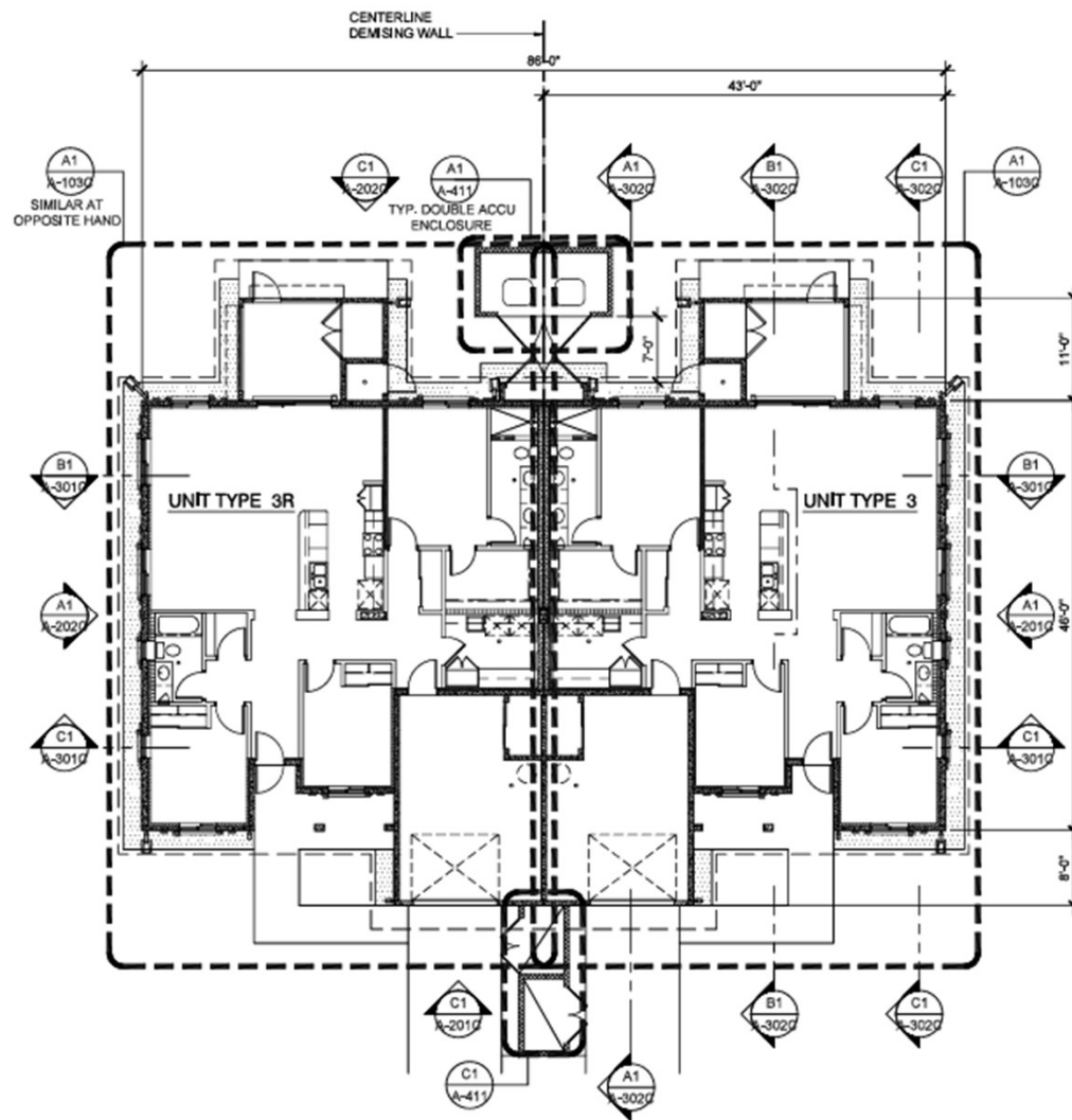
A1 FLOOR PLAN - BUILDING C SCALE: 1/8"=1'-0"
